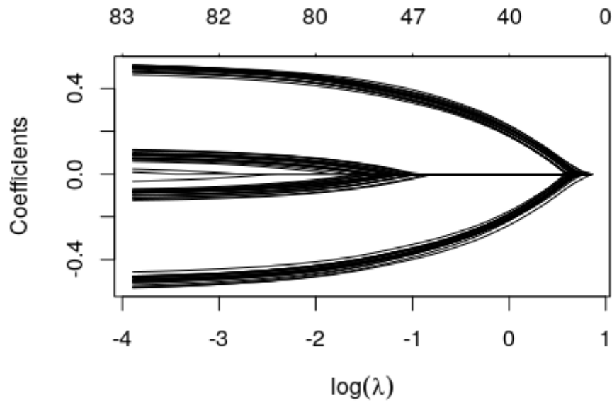
FIGURE 3.19 – Chemin des \beta
