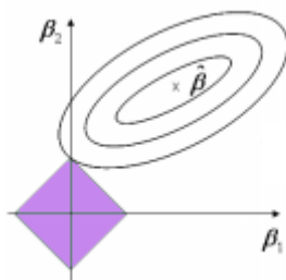
FIGURE 3.4 – Illustration de la contrainte LASSO
